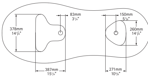
Underside View
